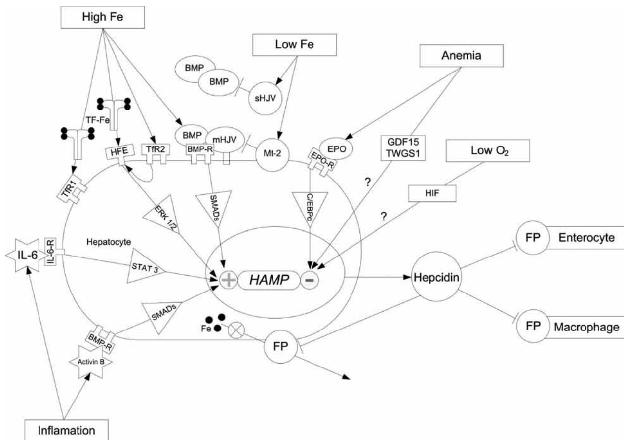
FIGURE 2. Regulation of hepcidin antimicrobial peptide ( HAMP ) expression. Iron abundance (high Fe) induces bone morphogenic proteins (BMPs) binding to their receptor (BMP-R) and SMAD-mediated induction of HAMP . Membrane hemojuvelin (mHJV) is a BMP co-receptor. Matriptase-2 (MT-2) is active in iron deficiency and hypoxia, inhibits BMP signal transmission. Soluble hemojuvelin (sHJV) is cleaved from HJV by furine convertase or type II transmembrane serin protease TMPRSS6. It competes with sHJV in BMP and has a negative effect on BMP signal transmission. High iron concentration causes binding of transferrin-iron complex (TR-Fe) to transferrin receptor 1 (TfR1). This binding displaces hereditary hemochromatosis protein (HFE) and signals HAMP induction, through interaction with transferrin receptor 2 (TfR2) and extracellular-signal-regulated kinases 1/2 (ERK1/2) signal pathway. Inflammation stimulates hepcidin production through two mediators, interleukin-6 (IL-6) and activin B. IL-6 binds to IL-6 receptor (IL-6-R) on hepatocyte and activates Janus kinase 2/signal transducer and activator of transcription 3 (JAK2/STAT 3) signal pathway. Activin B binds to BMP-R and activates SMADs. Both inflammatory mediators have a positive effect on HAMP expression. Anemia causes an increase in production of erythropoietin that binds to erythropoietin receptor (EPO-R) and down-regulates expression of signaling protein CCAAT/enhancer-binding protein α (C/EBPα) and hepcidin. The mechanisms of hypoxia inducible factor (HIF), growth differentiation factor 15 (GDF15) and twisted gastrulation (TWGS) as HAMP modulators is still controversial.
