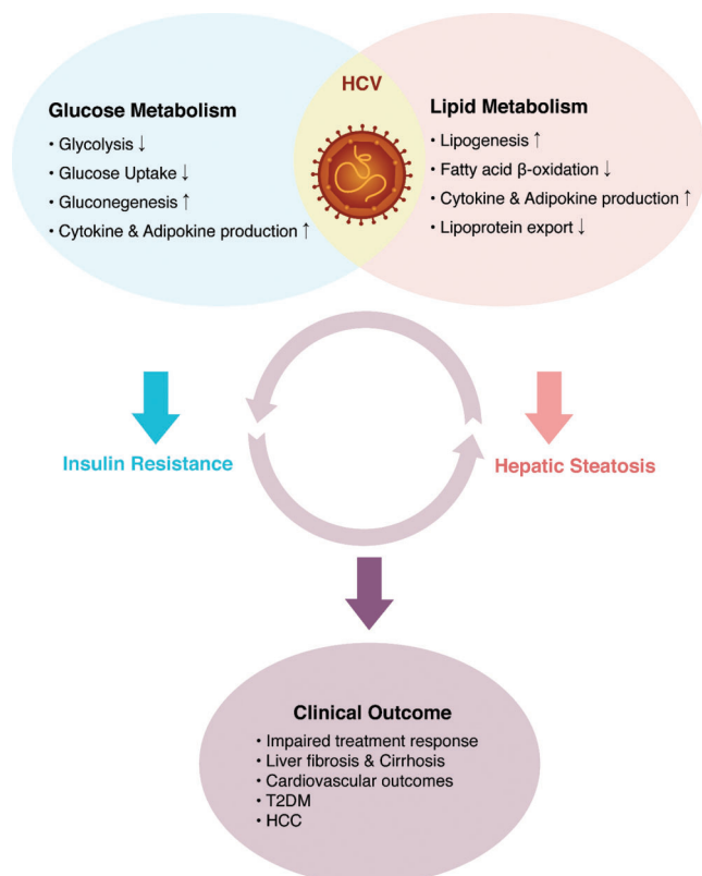
Fig. 1. Pathogenetic effects and outcomes of HCV infection.
